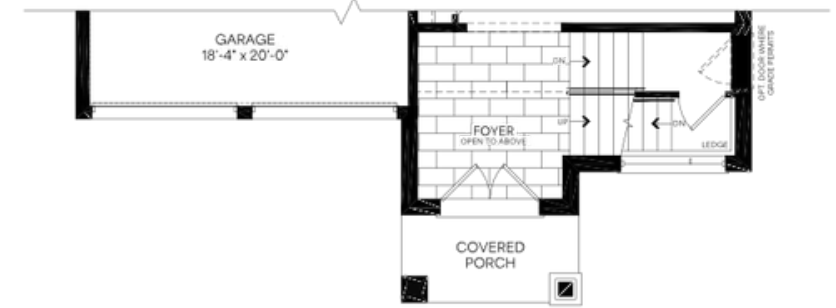
Main Floor Elevation C
