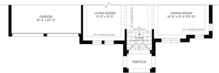
Main Floor Elevation B
