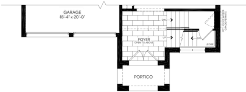
Main Floor Elevation B
