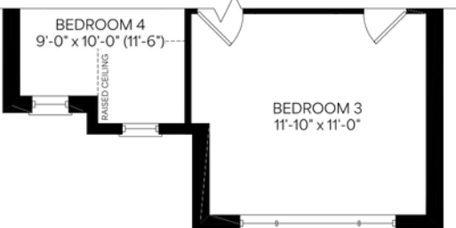
Second Floor Optional 4 Bedroom Plan Elevation C
