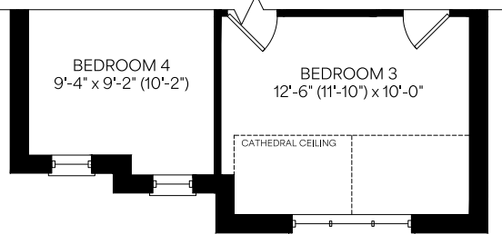
Second Floor Optional 4 Bedroom Plan Elevation B
