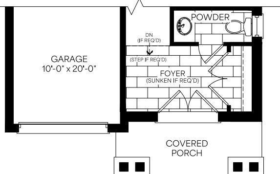
Main Floor Elevation C
